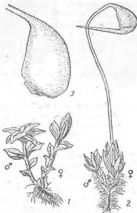
75-rasm. Funariya ( Funaria hydrometrica ) moxi:
