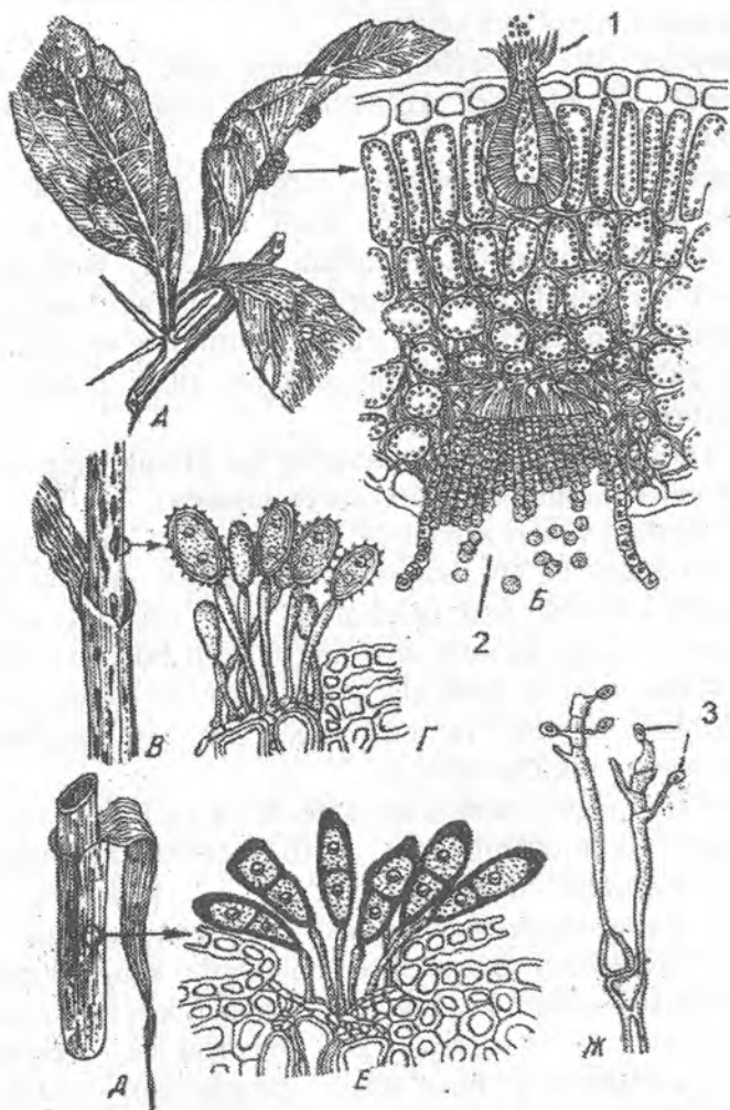
73-rasm. Bug'doyning ( Puccinia graminis ) chiziqli zang zamburug'i: A – kasallangan zirk usimligining bargi, B – piknidiy – 1 va esidiy – 2, V – kasallangan bug'doy poyasi, G – uredo-sporalar to'plami, D – teleytosporali bug'doy poyasi, E – teleytosporalar to'plami, J – ungan teleytospora, bazidiyasporalar bilan.
