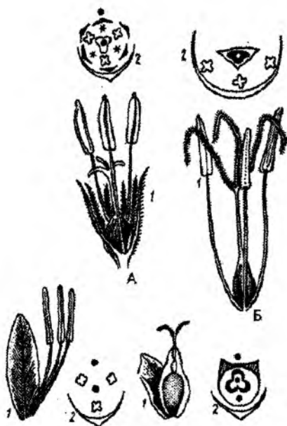
108-rasm. Qiyogdoshlar (Cyperaceae):
