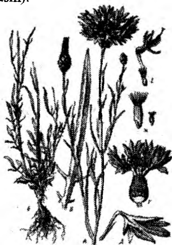
106-rasm. Bo'tako'z ( Centaurea depressa M.B.): A – B – umumiy kurinishi, V – bargi, G – bñyiga kesilgan savatcha tãpgul, D – chetki varonkasimon gul, E – irtangi naychasimon gul, J – meva
