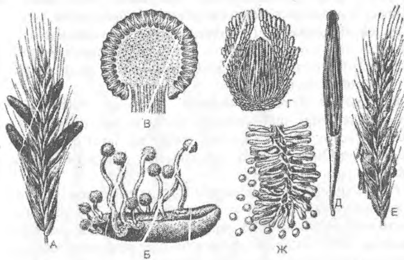
71-rasm. Shoxkuya ( Claviceps purpurea ) zamburug'i: A – shoxkuya bilan zararlangan javdardagi boshog'i, B – sklerotsiyning o'sishi, V – stromaning boshcha orqali bo'yama kesimi, G – peritetsiy so'mkasi bilan, D – ipsimon sakkiz sporalik xaltacha, E – gullayotgan boshog'dagi shudring tomchisi, J – konidiyasporasi
