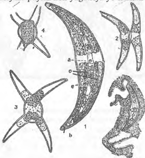
60-rasm. Klosterium ( Closterium ): 1 – a – yadro, o – xromotofora, e – perinoidlar, 2 – vakuolasi, 2 – 3 – 4 – kŕpayish (konyugatsiya)
