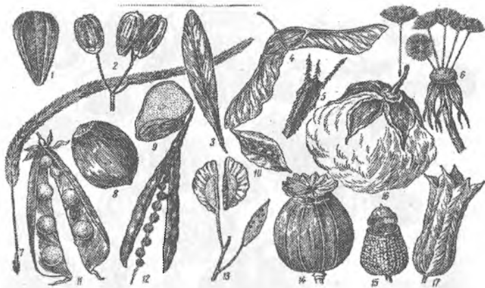
54-rasm. Quruq mevalar: 1 – pista, 2 – qo‘sh pistacha, 3 – qanotchali, 4 – qo‘shqanotli, 5 – ilashuvchi pistacha, 6 – uchuvchi pistacha, 7 – uchuvchi don, 8 – yong‘oq, 9 – don, 10 – bargcha, 11 – dukkak, 12 – qo‘zoq, 13 – qo‘zoqcha, 14–15–16 –ko‘sak, 17 – ochiladigan ko‘sak.
