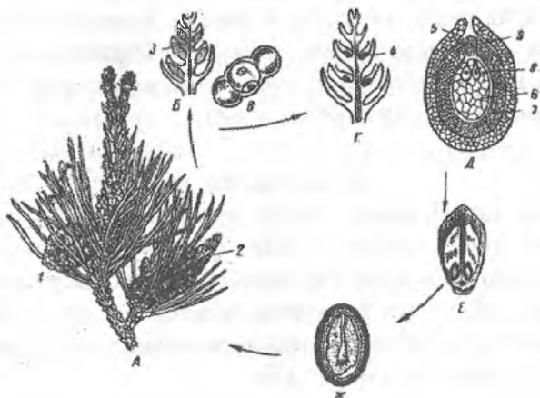
79-rasm. Oddiy qarag‘ay ( Pinus silvestris ):
