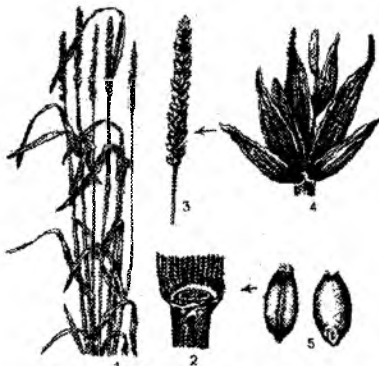
111-rasm. Yumshoq bug'doy ( Triticum aestivum ) qiltiqsiz: 1 – ÷simlik tipi, 2 – barg qini, quloqchasi bilan, 3 – murakkab boshog' tup guli, 4 – boshog'qcha, 5 – don mevasi
