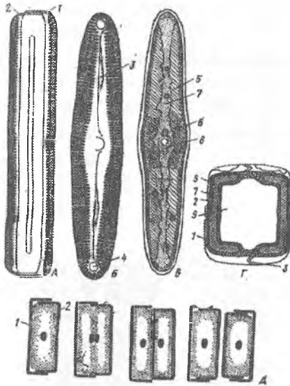
62-rasm. Diatom suvtlaridan Pinnulariya (Pinnularia): A – yuza tomonidan, B – tep tomonidan, V – uzunasiga kesimi, G – kundalang kesimi, D – vegetativ topaych; 1 – epitika, 2 – gipotika, 3 – chok, 4 – tuguncha, 5 – xromatofor, 6 – perenoid, 7 – sitoplazma, 8 – yadro, 9 – vakuol.
