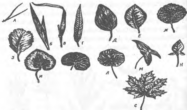
40-rasm. I-oddiy barglar: A – ninasimon, B – xanjarsimon, V – lentasimon, G – nashtarsimon barg, D – tuxumsimon, E – ovalsimon, J – yumaloq, Z – teskari tuxumsimon, I – yuraksimon, K – buyraksimon, L – qalqonsimon, M – N – nayzasimon, S – panjasimon bo‘lingan. II – murakkab barglar: A – uch bargchali murakkab barg, B – panjasimon murakkab barg, V – toq patsimon murakkab barg, G – qo‘sh yoki ikki marta patsimon murakkab barg,
