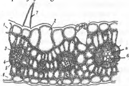
42-rasm. Makkajo'xori bargining ko'ndalang kesimi: 1 – ustki epidermis, 2 – harakatlantiruvchi hujayralar, 3 – mezofill hujayralar, 4 – o'tkazuvchi bog'lam: a – ksilema, b – floema, 5 – o'rab turuvchi hujayralar, 6 – ostki epidermis, 7 – dag'al tuk.
