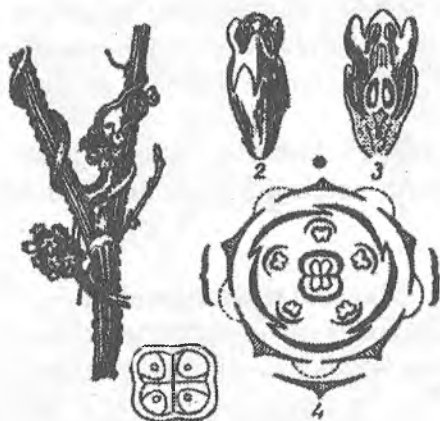
86-rasm. Zarpechak ( Cuscuta campestris ):
