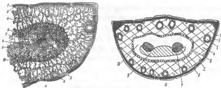
44-rasm. Qarag'ay bargining ichki tuzilishi: 1 – epidermis, 2 – ustitsa (og'izcha), 3 – gipoderma, 4 – qatlamli parenxima, 5 – smola yo'llari, 6 – endoderma, 7 – ksilema, 8 – floema (7 – 8 – o'tkazuvchi bog'lam), 9 – sklerenxima, 10 – parenxima.
