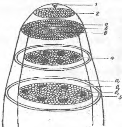
10-rasm. Hosil qiluvchi to'qima sxemasi: 1 – ini-sial hujayra, 2 – promeristema, 3 – meristema, 4 – pro-kambiy, 5 – kambiy. a – dermatogen, b – periblela, v – pleroma, a 1 – epidermis, b 1 – birlamchi po'stloq, v 1 – markazy silindr.
