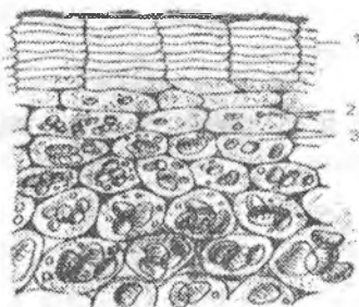
13a-rasm. Kartoshka tunganigidagi g‘amlovchi parenxima: 1 – po‘kak,
