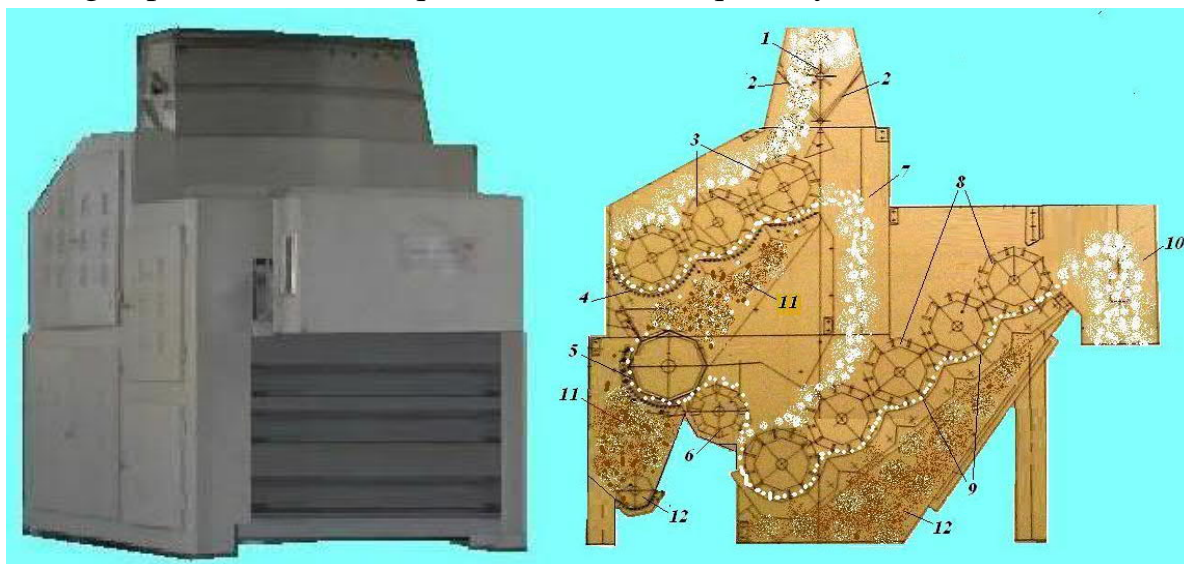
12-rasm. MQZT -2400 rusumli paxta tozalagichining ko'ndalang qirqimi
