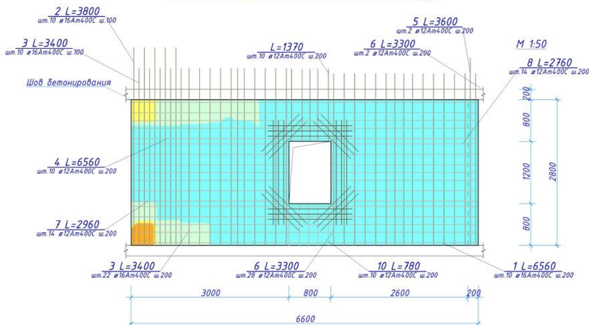
63-rasm. Tuynugi hoshiyalanishi bilan konstruksiyalangan diafragma
