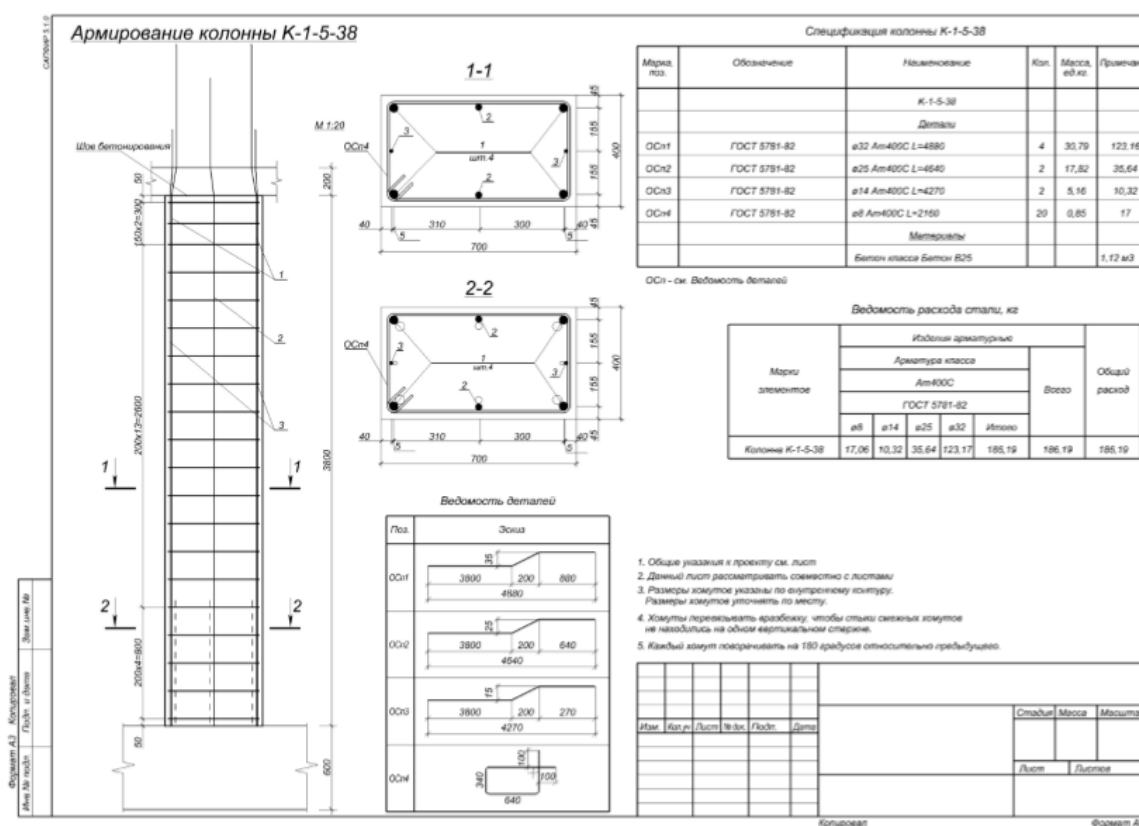
35–rasm. Ustunlarni armaturalash chizmasi
