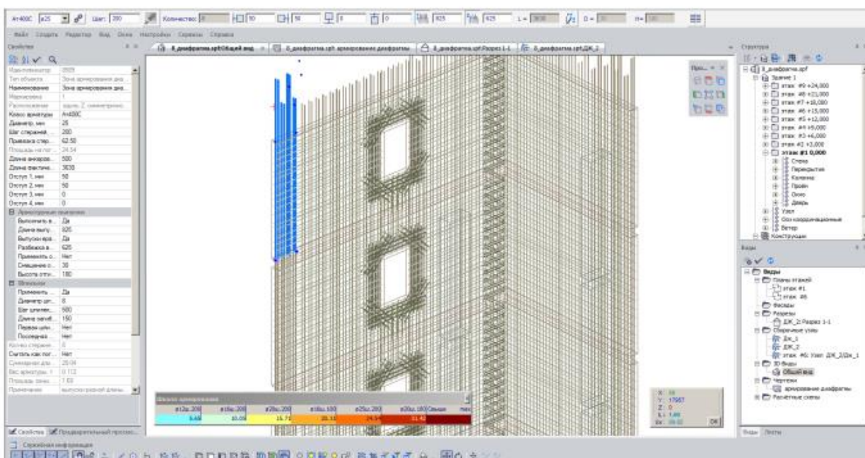
73-rasm. Loyihalangan armaturalashning 3D ko‘rinishi
