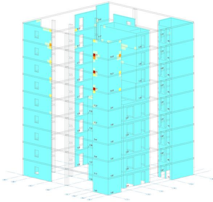
48-rasm. Hisobiy armaturalashni vizuallashtirish.
