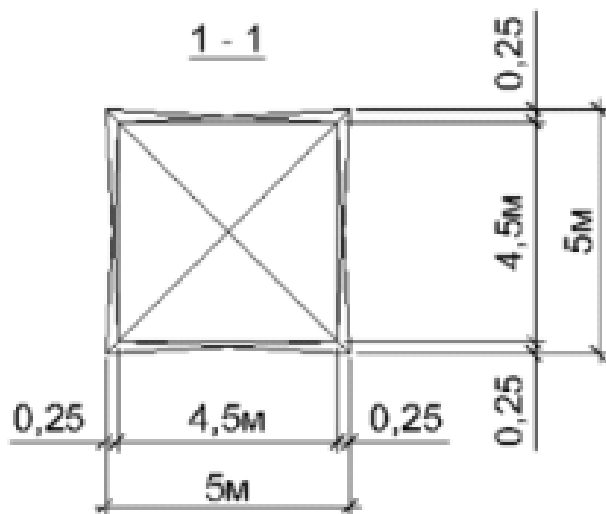
78-rasm. Metall minora sxemasi
