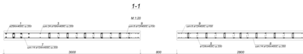
68-rasm. DJ_2 diafragmani markalash
