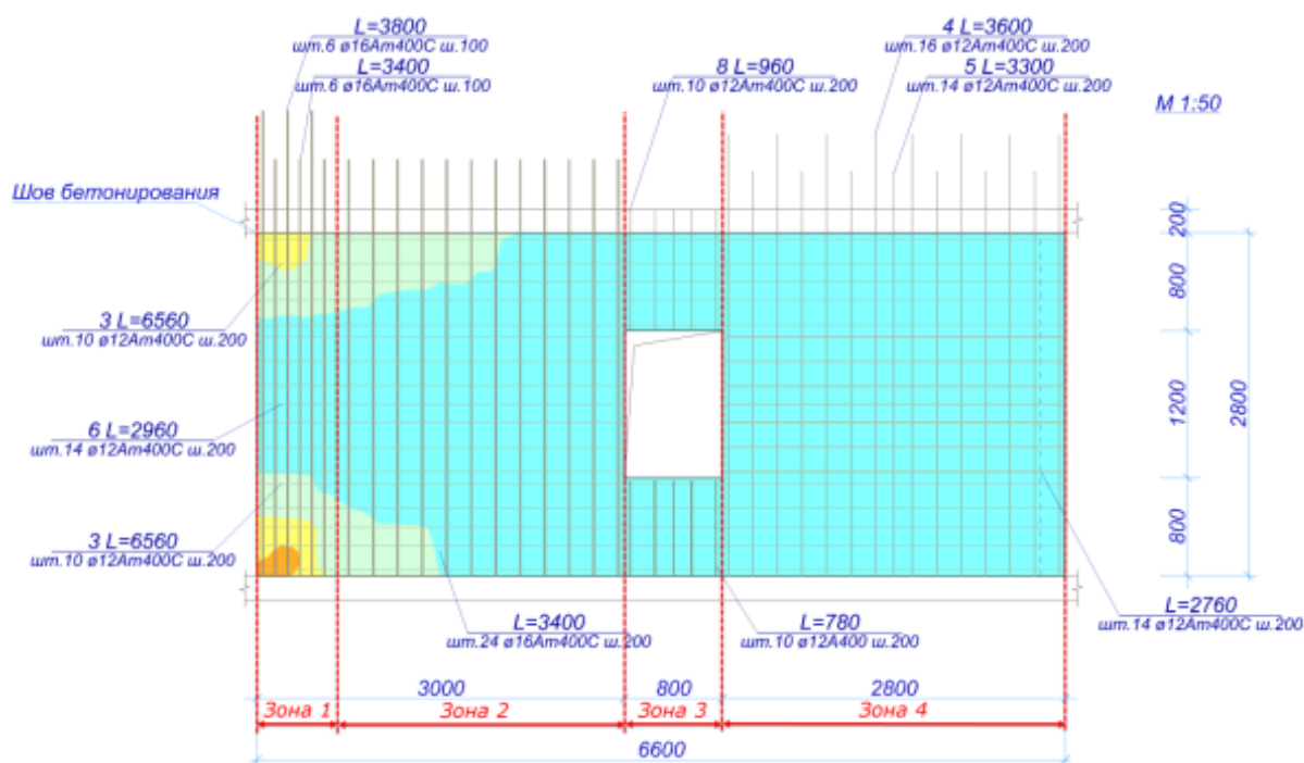
13.15-rasm. Armaturalash zonasining joylashishi
