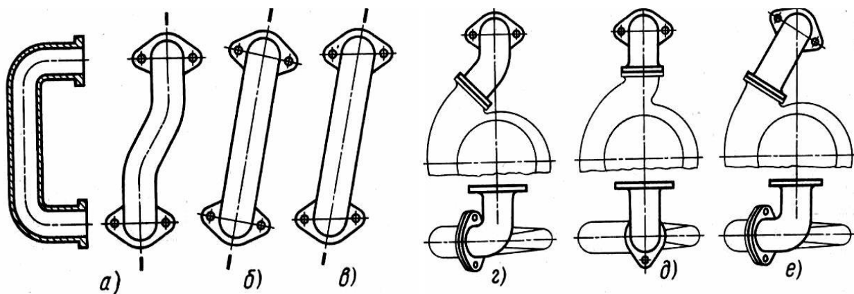
2.7-rasm. Egri chiziqli patrubkalarning shaklini soddalashtirish
