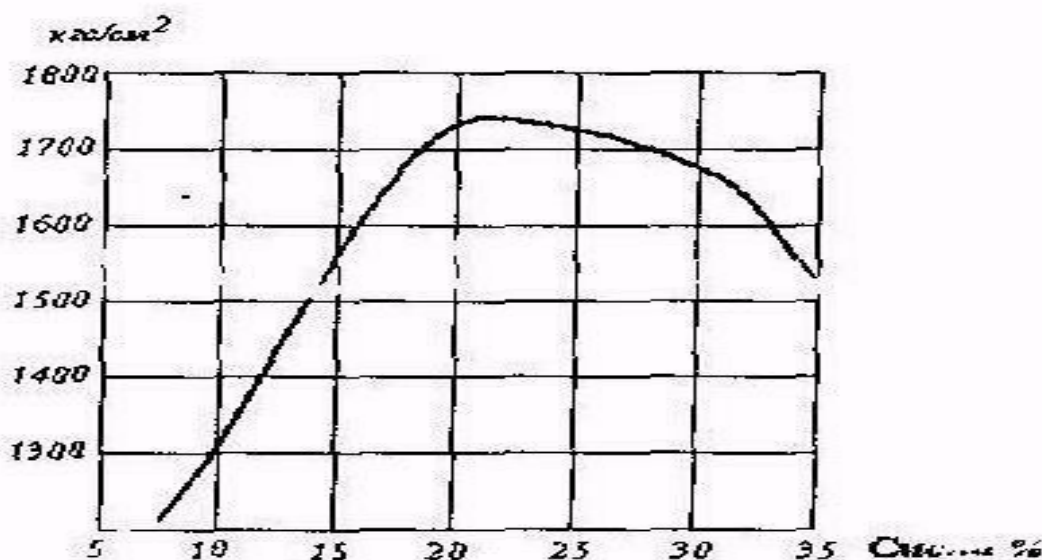
2.4-rasm. Toshko'mir smolasining uglerod-grafit materialning cho'zilishdagi mustahkamligiga ta'siri.
