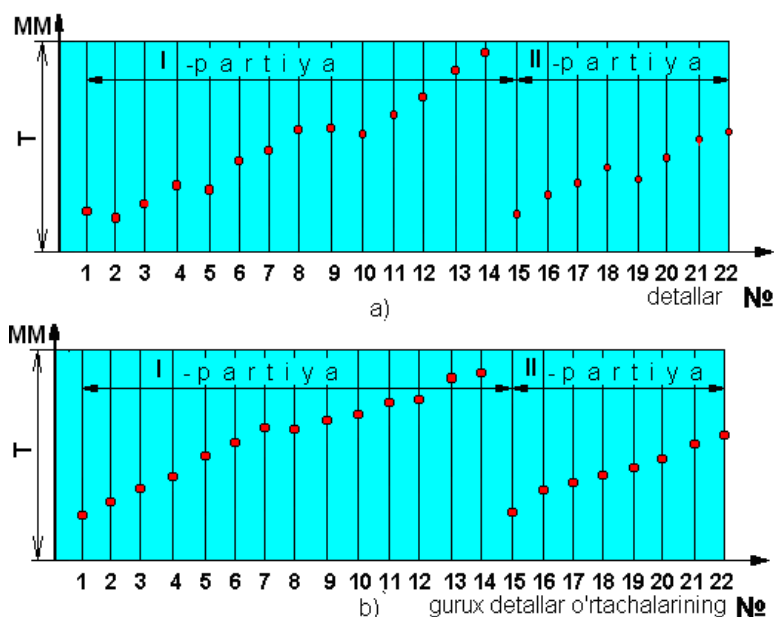
8-rasm. Nuqtali diagrammalar
