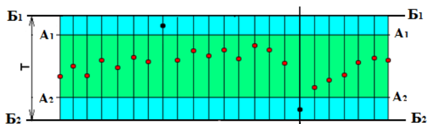
9-rasm. Statistik nazorat uchun nazorat diagrammasi
