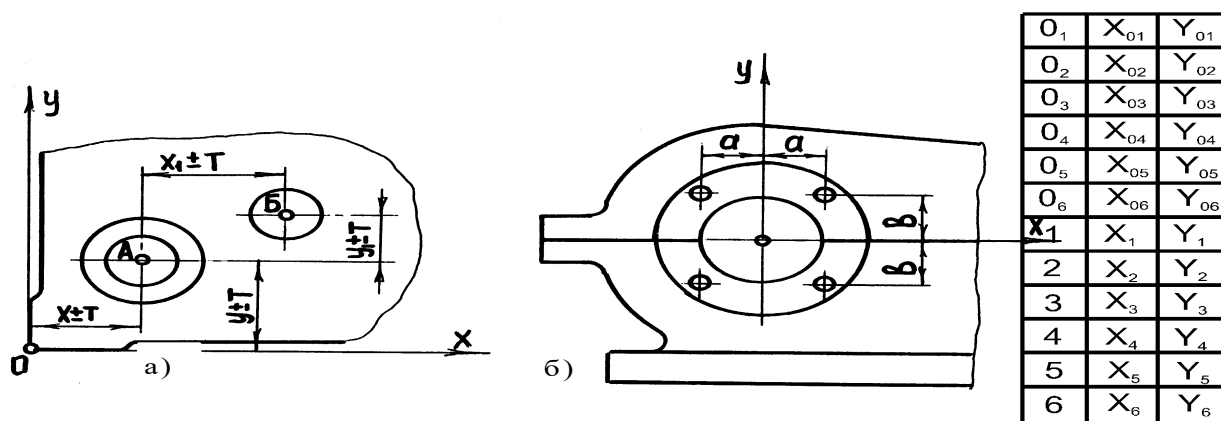
Rasm 8. RDB stanogi uchun detal chizmasida o'lchamlar
