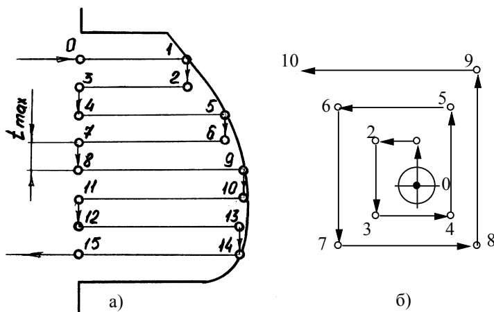
3 - rasm. Frezalashdagi traektoriyalar: a) zigzagsimon; b) spiralsimon
