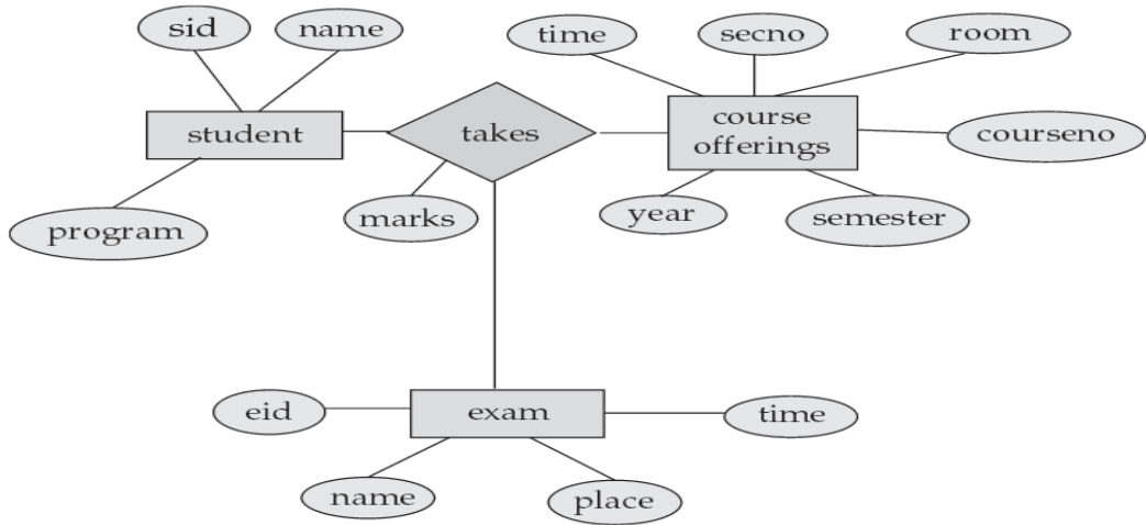
Figure 6.3 E-R diagram for marks database.
