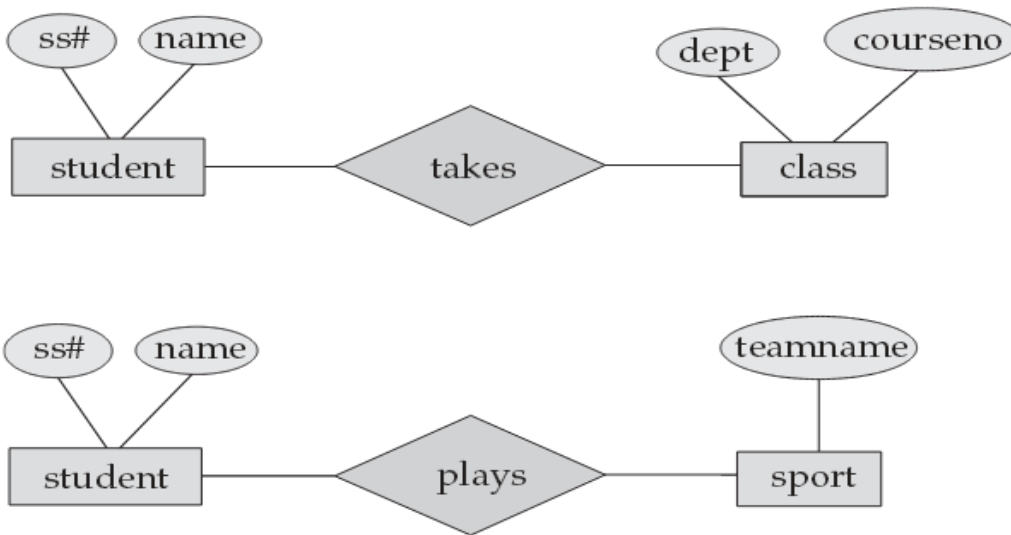
Figure 6.6 E-R diagram with entity duplication.
