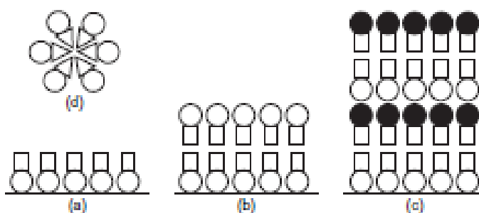
FIGURE 8.8 Langmuir-Blodgett films. (a) A monolayer; (b) a bilayer; (c) a Y-type multilayer. The circles represent the polar heads and the squares the apolar tails of the amphiphilic molecule. (d) A micelle, which can form spontaneously upon dispersal in water if the amphiphilic molecules have a smaller tail than the head (see Section 8.2.9).
