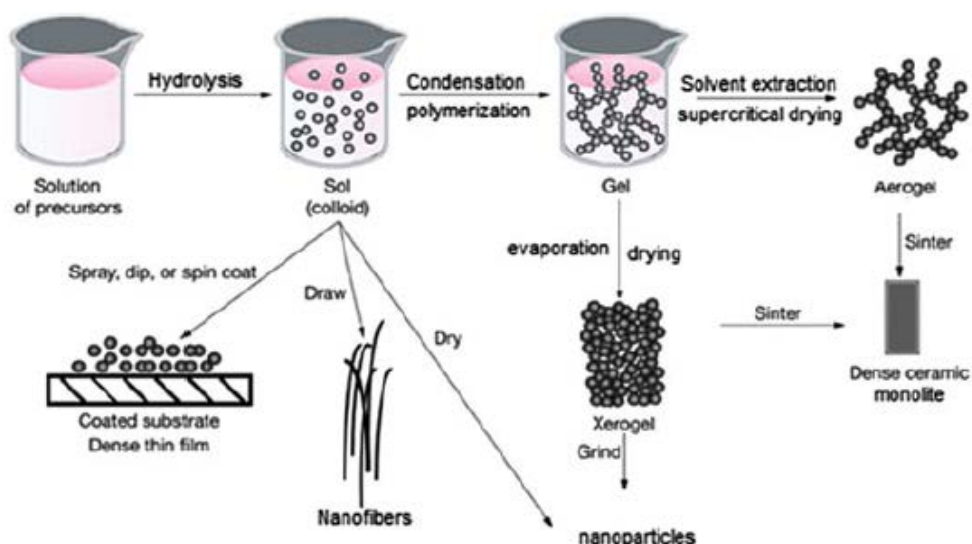
Fig. 2.10 Schematic diagram of sol-gel method and its nanomaterials products
