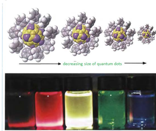
Color of CdSe - CdS colloids is a function of quantum dots sizes
