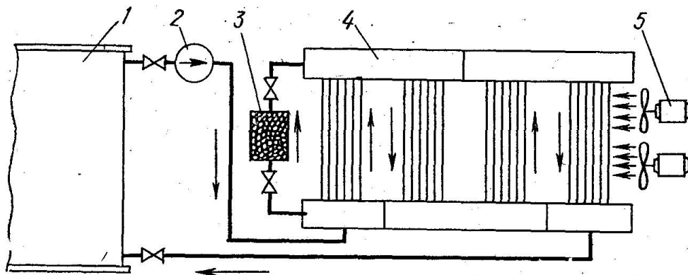
2-rasm. III tizimi sovitgichning prinsipial sxemasi: 1–transformator baki; 2–elektr nasosi; 3- adsorb filtr; 4-sovitkich; 5-puflash ventilyatori.
