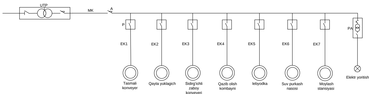
2.2-rasm. Yer osti uchastkasi elektr ta'minoti tuzilish sxemasi UTP-uchastka transformator podstansiyasi, A-avtomat, P-puskateli, MK-magistral kabel, EK-egiluvchan kabel, PA-puskovoy apparat
