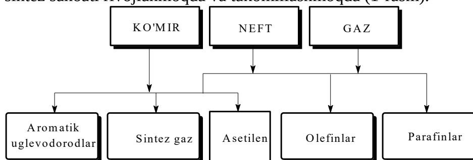
1-rasm. Organik sintez sanoati xomashyolari
