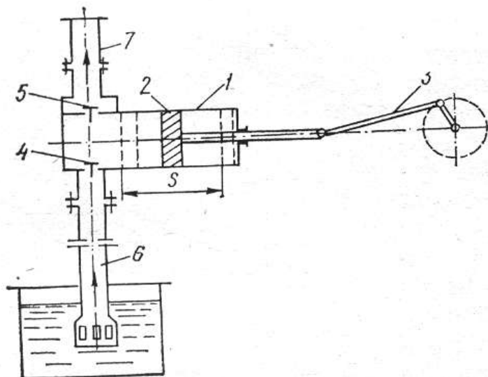
2 - rasm. Oddiy gorizontal holatdagi porshenli nasos
