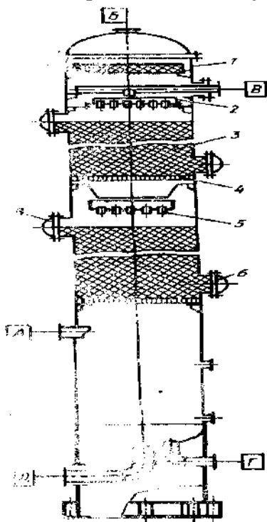
40-rasm. Nasadkali absorber
