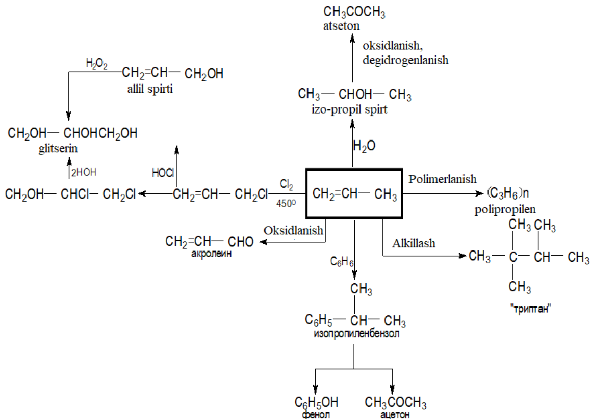
75-rasm. Propilenning neftkimyo sintezda isglatilishi
