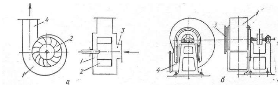
4 – rasm. Markazdan kochma ventilyator.
