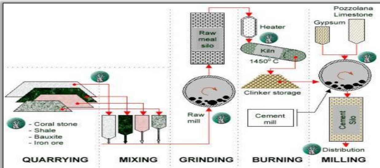
17-rasm. Porland sement ishlab chiqarish tizimi
