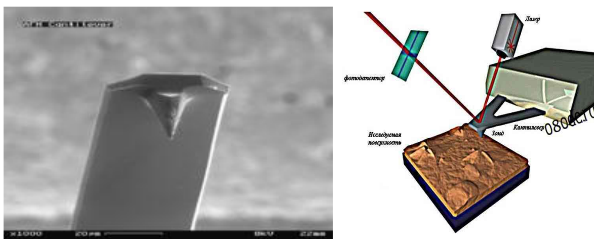
15- рasm. Микрозondning ko‘rinishi (A) va ishlash prinsipi (B).
