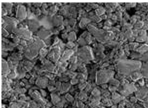
5-Rasm. B. 2000X kattalashtirilgan kaliy xloridi changi minerallarining rasmi.
