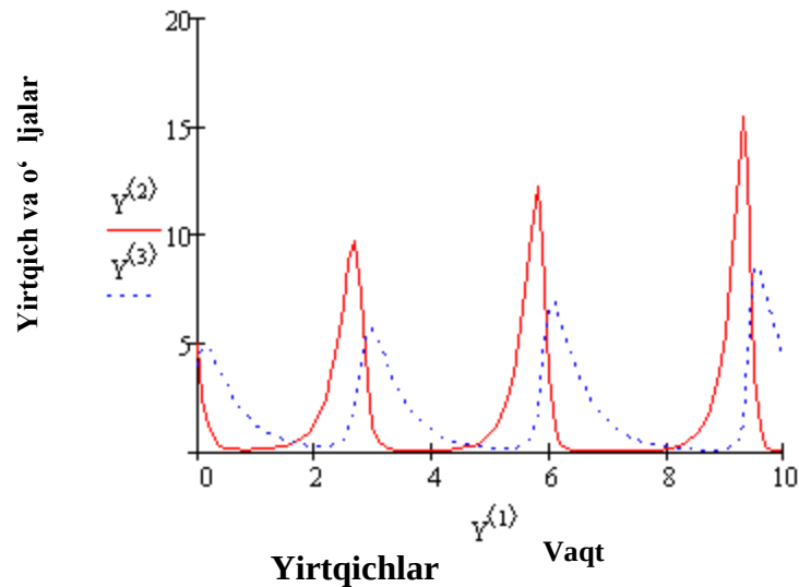
9.7-rasm. Manfiy koeffitsientli ( \alpha = -0.04 ) raqobat asosida Volter-Lotka modelining evolyusiyasi, yirtqichlarning boshlang'ich soni x^0_1 = 500 , o'ljalarining soni esa x^0_2 = 400 , a = 4 , b = 2,5 , c = 2 , d = 1 .
