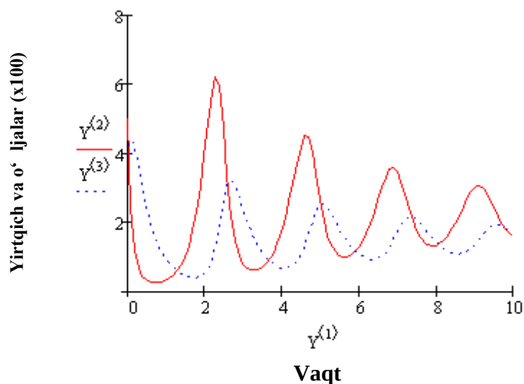
9.5-rasm. Volter-Lotka modelining musbat koeffitsientli ( \alpha=0.1 ) raqobat bilan evolyusiyasi, yirtqichlarning boshlang'ich soni x_1^0=500 , o'ljalarniki esa x_2^0=400 , a=4, b=2.5, c=2, d=1 .
