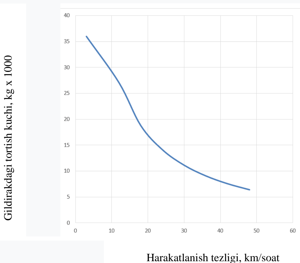
2-rasm. Tortish kuchining harakat tezligiga bog'liqlik grafigi
