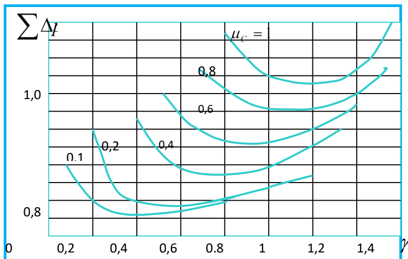
11.2–rasm. Yuklanish momentining turli qiymatlari uchun asinxron motor (nominal quvvati R_N = 100 kVt va 2R = 4 ) umumiy quvvat isroflarining stator chulg’ami kuchlanishiga bog’liq ravishda o’zgarishi tavsiflari
