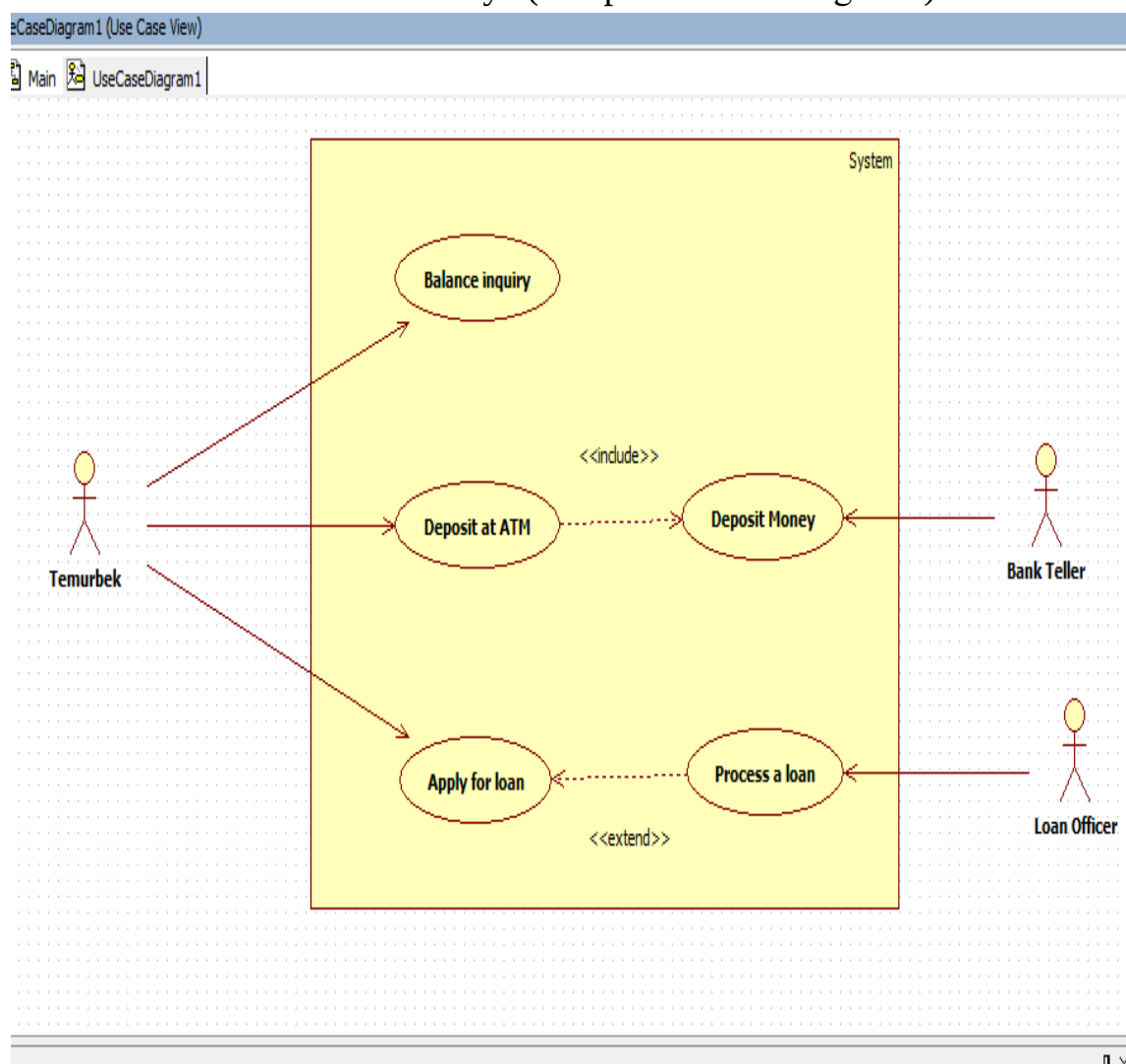
1.5-rasm. Loyihaning Use Case diagrammasi
