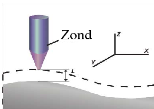
9-rasm. STMning ishlash sxemasi
