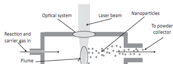
Figure 4.11 Schematic drawing of the experimental setup for nanoparticle synthesis applying laser ablation. The pulsed laser beam is focused at the surface of the precursor target that may be a metal or an oxide. The high-intensity laser beam causes a plume, a supersonic jet of evaporated
