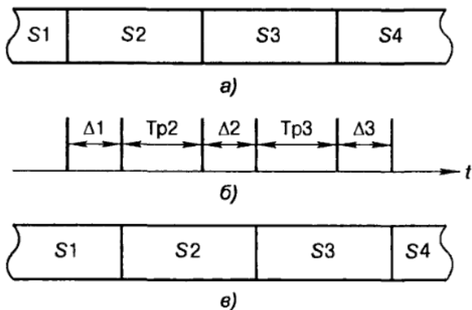
2.13-rasm. Himoya intervallarining shakllantirilishi
