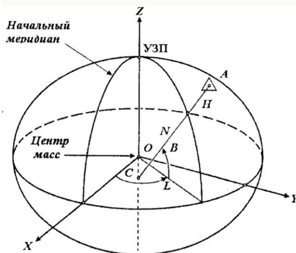
3.1 rasm. Krasovskiy ellipsoidi
