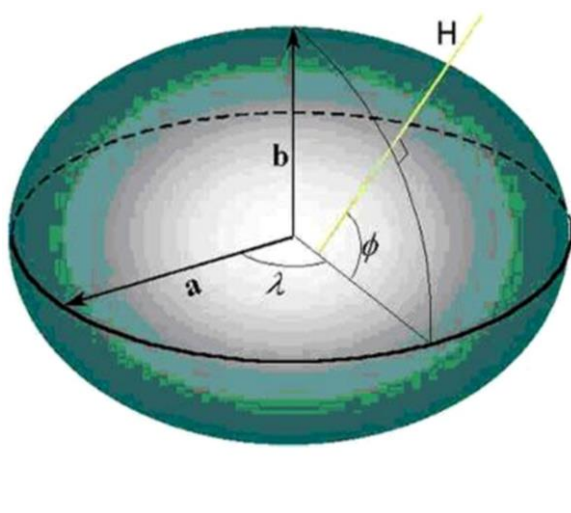
3.1 rasm. Krasovskiy ellipsoidi
