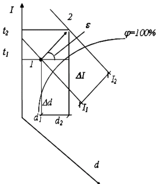
1.3-rasm. I-d -diagrammasida havoning holatini o‘zgarishini ko‘rsatish va yunalishini aniklash
