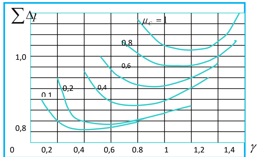
11.2–rasm. Yuklanish momentining turli qiymatlari uchun asinxron motor (nominal quvvati R_N = 100 kVt va 2R = 4 ) umumiy quvvat isroflarining stator chulg’ami kuchlanishiga bog’liq ravishda o’zgarishi tavsiflari
