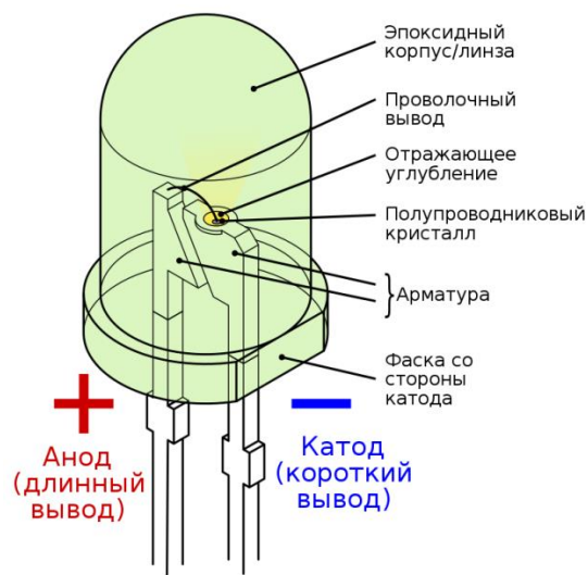
Rasm. Nurdiod tuzilishi
