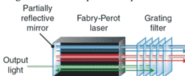
Rasm. 2. Filtrlar bilan sozlanishi lazerlar dispersion panjaralar asosida
