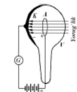
10.8-rasm. Fotoelement.
