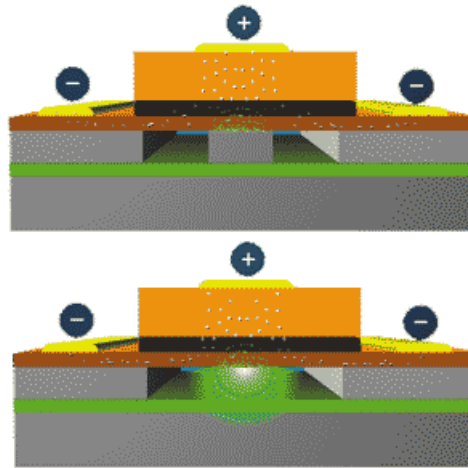
Rasm. 10. Gibridd kremniy lazerning tuzilishi
