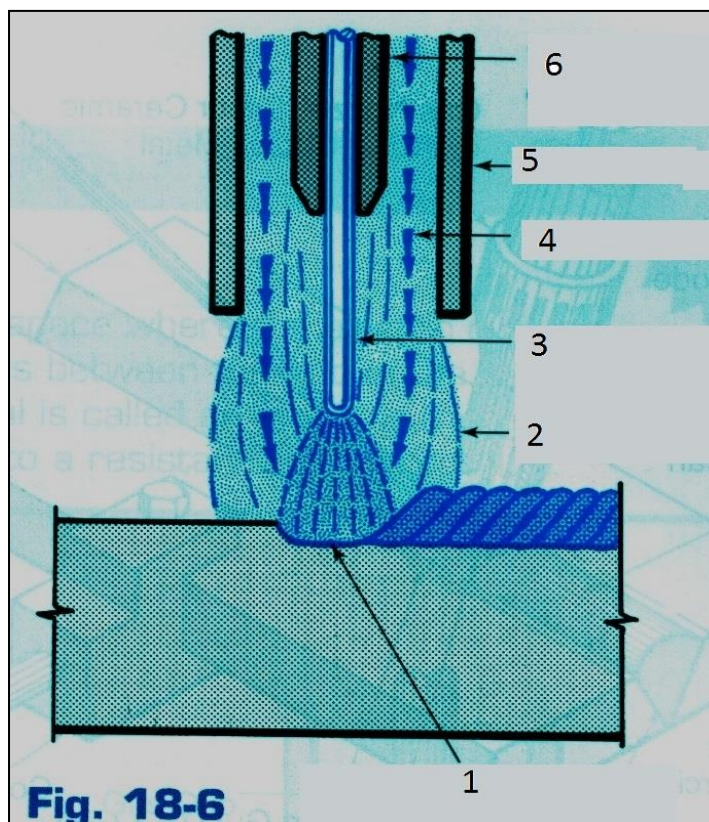
1.6 –rasm. Himoya gazlar muhitida payvandlash jarayonining chizmasi: 1 – yoy; 2 – himoya atmosferasi; 3 – elektrod; 4 – himoya gazi; 5 – soplo 9 .
