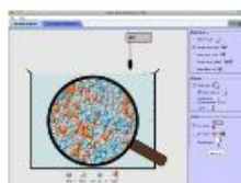
Acid-Base Solutions
