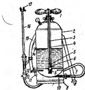
2.70-rasm. Avtomaksning sxematik ko‘rinishi: 1- shtok dastasi, 2-rezervuar, 3- nasos silindri, 4- porshen shtoki, 5- porshen buferi, 6- porshen, 7-shlang, 8- haydaydigan klapan, 9- karkas, 10- shtutser, 11- tasma, 12-bekitadigan kran, 13- filtr, 14- kontrol sath probkasi, 15- kamar, 16-chiqaruvchi metall naycha, 17-qo‘sh rojokli changlatgich
