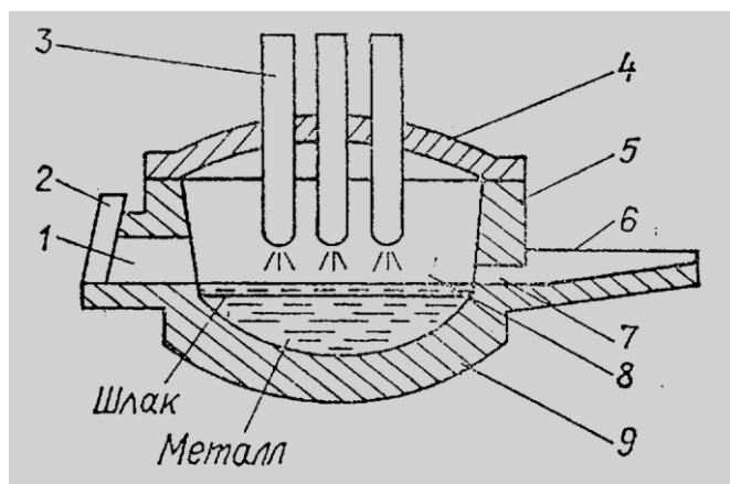
Yoyli pechning sxema:
