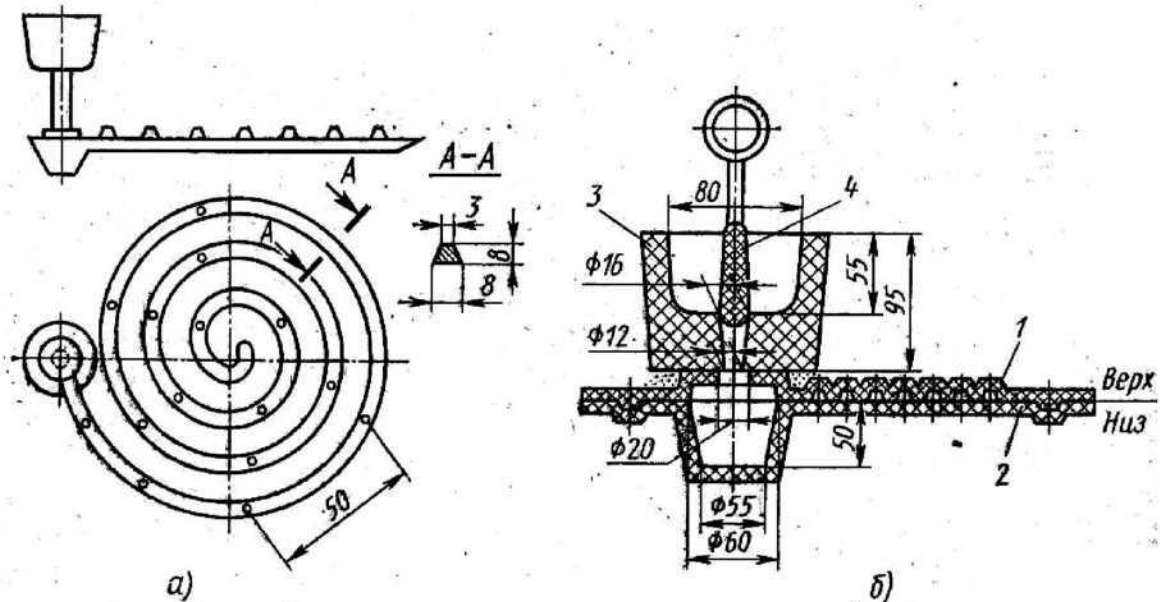
Okuvchanlik aniklash uchun spiralli namuna (a) va kuyma shakl (b): 1-2-pastki va yukorigi yarim shakllar; 3-kuyish chashkasi, 4-grafitli tikin
