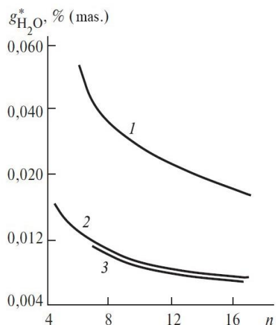
2.1-rasm. t = 20\text{ }^{\circ}\text{C} va p_s = 0,101\text{ MPa} da individual uglevodorodlarda, molekuladagi uglerodlar soniga qarab, suvning maksimal eruvchanligi: 1-aromatik, 2-naftenli, 3- parofinli
