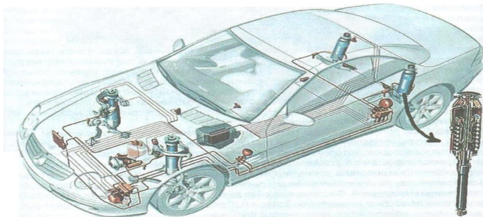
4.19-rasm. Mercedec avtomobilining faol osmasi
